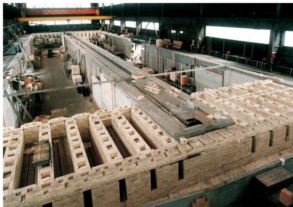
Figure 1: Open top ring type furnace under construction
