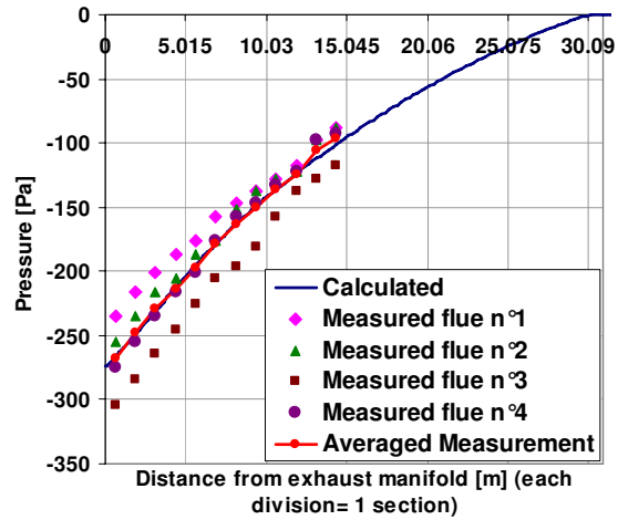
Figure 11: Comparison of measured and calculated draught profiles inside the flues at preheat
